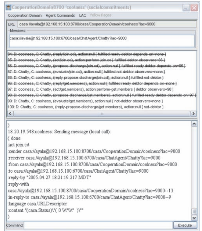
Figure 7: A CASA CD showing a conversation with another agent requesting to join the CD
