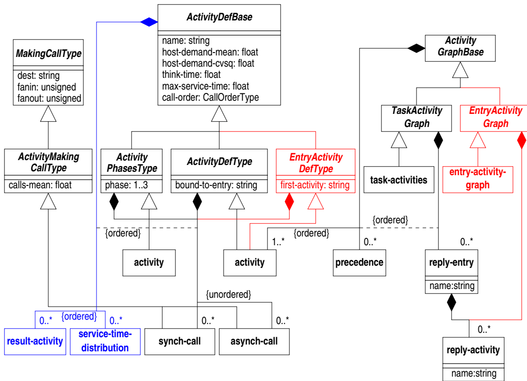
Figure 3.6: Schema diagram for the type ActivityGraphBase
