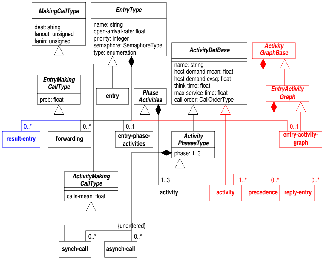
Figure 3.5: Schema for type EntryType .
