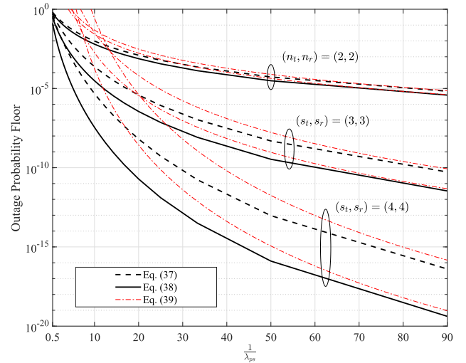
FIGURE 4. The direct-transmission outage probability floor for both TAS strategies versus the inverse of \lambda_{ps} for different antenna configurations while \lambda_{ss} = 1 , \lambda_{sp} = 0.1 , Q_{th} = -0.1 dB and \varepsilon_p = 0.01 are fixed.
