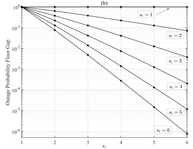
FIGURE 3. (a): The direct-transmission outage probability opF_{s,snr}^1 and opF_{s,snr}^1 at a certain threshold \Phi_s = 2^2 - 1 versus the primary system SNR ratio P_p/N_0 while having \lambda_{ss} = 1 , \lambda_{sp} = \lambda_{ps} = 0.1 and Q_i = 0 dB fixed. (b): The outage probability floor gap between (37) and (38), appearing when P_p/N_0 \rightarrow +\infty , is calculated for different antenna configurations.
