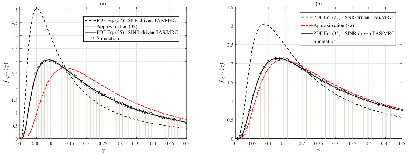
FIGURE 1. The MRC combiner output SINR PDFs (27) and (35) when the SNR and SINR-driven TAS/MRC strategies are adopted, respectively. Both PDFs are compared against the one generated according to approximation (32). For both figures, we have taken \lambda_{ss} = \lambda_{sp} = \lambda_{ps} = 1 , P_p/N_0 = 10\text{dB} and Q_i = -5\text{dB} as practical system settings that can arbitrary be modified. The figure on the left (a) is generated for s_t = 5 and s_r = 2 , whereas the figure on the right (b) is generated for s_t = 2 and s_r = 5 . The index s_1 in f_{\gamma_{s_1}^{s \rightarrow s}}(\gamma) equals either \hat{s}_1 or \bar{s}_1 depending on the TAS/MRC strategy being utilized.
