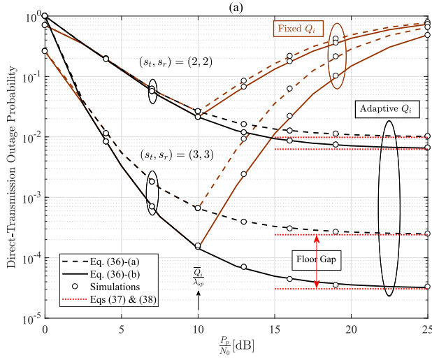
FIGURE 3. (a): The direct-transmission outage probability opF_{s,snr}^1 and opF_{s,snr}^1 at a certain threshold \Phi_s = 2^2 - 1 versus the primary system SNR ratio P_p/N_0 while having \lambda_{ss} = 1 , \lambda_{sp} = \lambda_{ps} = 0.1 and Q_i = 0 dB fixed. (b): The outage probability floor gap between (37) and (38), appearing when P_p/N_0 \rightarrow +\infty , is calculated for different antenna configurations.
