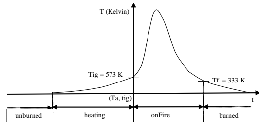
Figure 5: Simplified temperature curve of a cell's behavior
