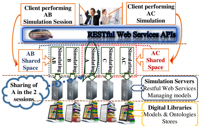
Figure 4. Simulation sessions with model sharing.
