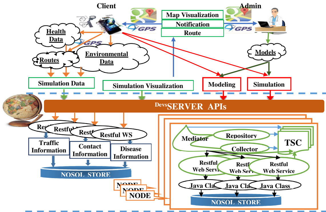
Figure 5. DevsServer architecture.
