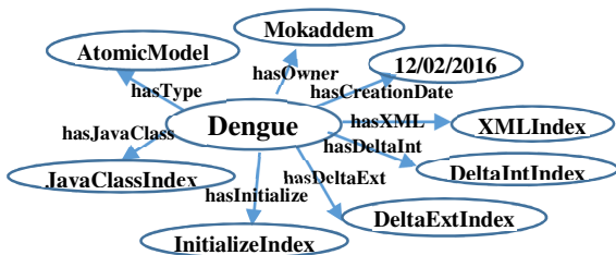
Figure 6. Graph model of a DEVS Dengue example.
