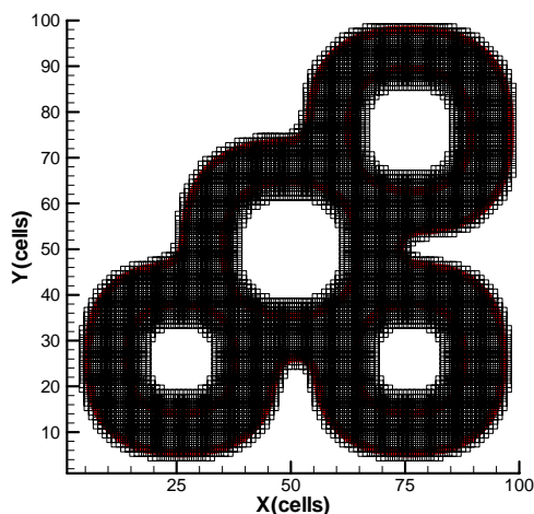
Figure 9: Activity tracking
