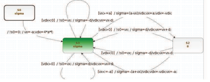
Figure 8: Triangular wave
