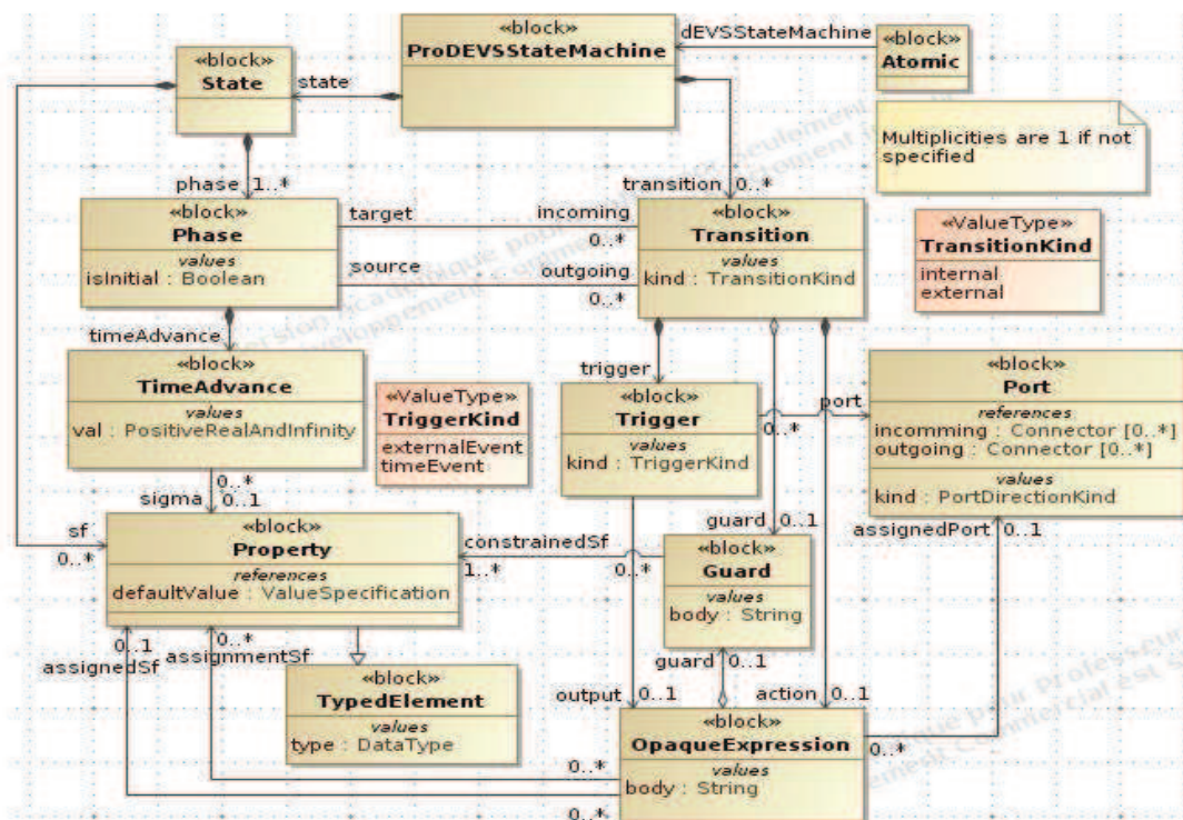
Figure 3: ProDEVS StateMachine
