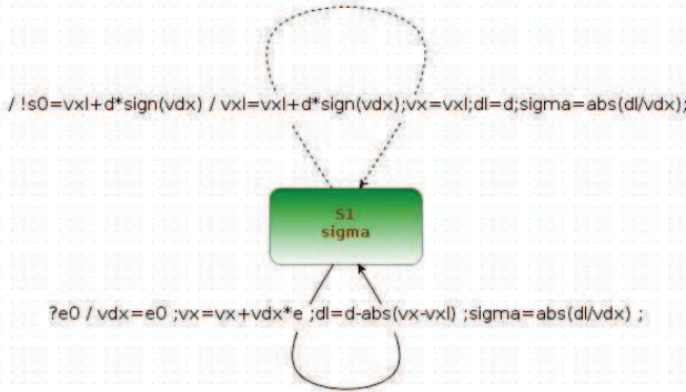
Figure 7: Quantized integrator
