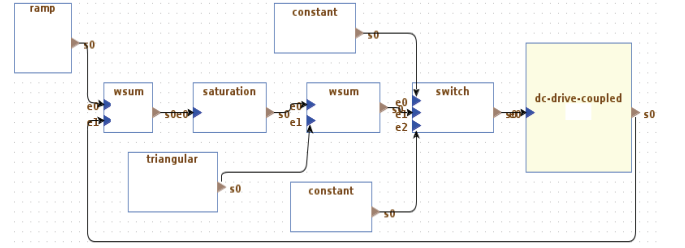
Figure 9: dc-drive model level 0
