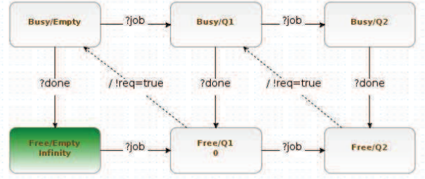
Figure 6: Atomic component BUF with six phases for a buffer with capacity of 2 (taken from [14] page 465).
