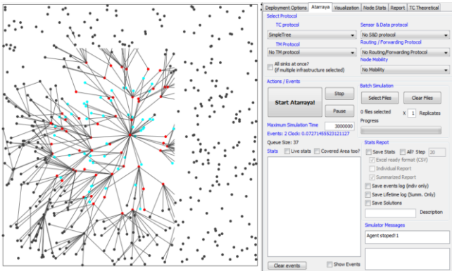
FIGURE 8. Atarraya simulation panel.
