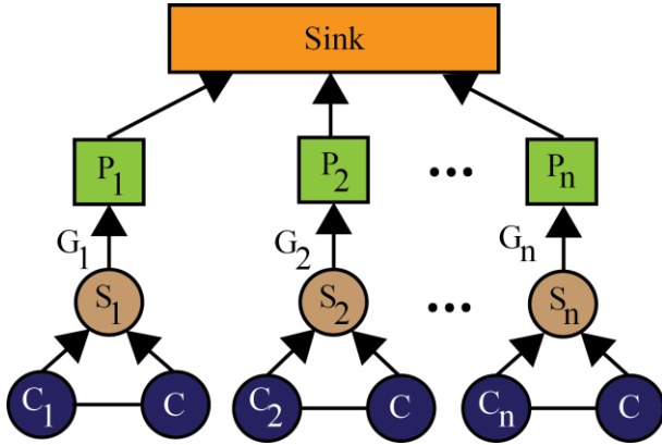
FIGURE 4. Illustration of a network model.
