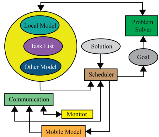
FIGURE 3. A Typical agent structure.
