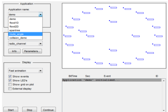
FIGURE 7. User interface of Prowler.
