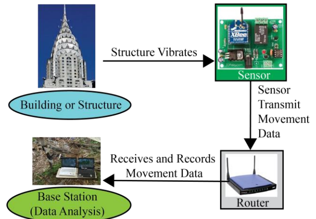
FIGURE 2. Illustration of a WSN for structural health monitoring.
