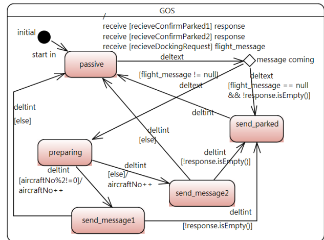
Figure 13. State Machine Diagram of GOS
