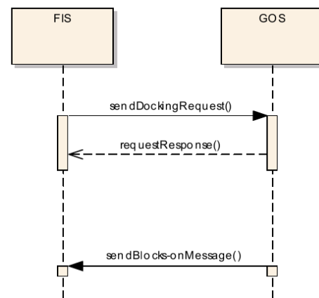
Figure 12. Service Choreography between FIS and GOS
