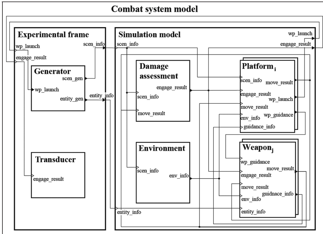
Figure 4. Graphical notation of Combat system model using DEVS diagram.
