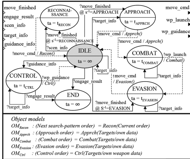
(c) Actor atomic model
