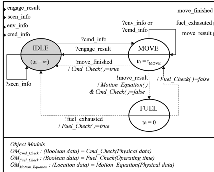
(c) Actor atomic model
