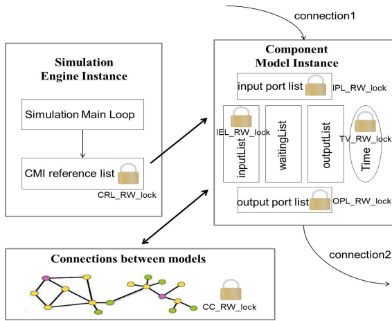
Fig. 3 Locks used in Ivy
