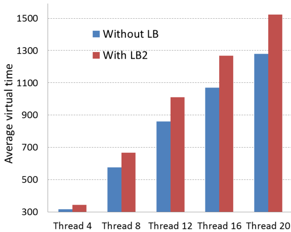
Fig. 8 Experiment results of common simulation
