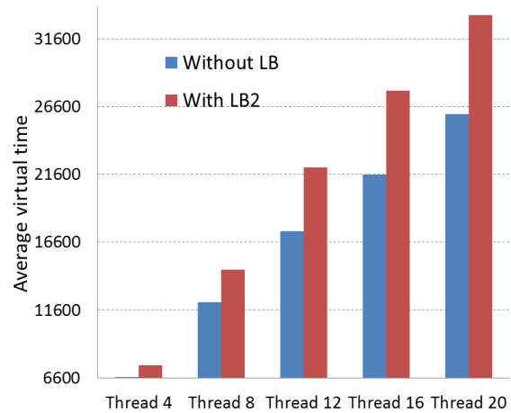
Fig. 9 Experiment results of variable structure simulation
