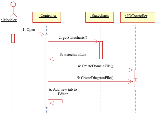
Figure 7. Sequence diagram to open a model
