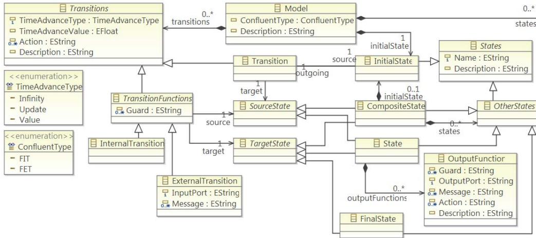
Figure 2. An Ecore DEVS meta-model using Statecharts
