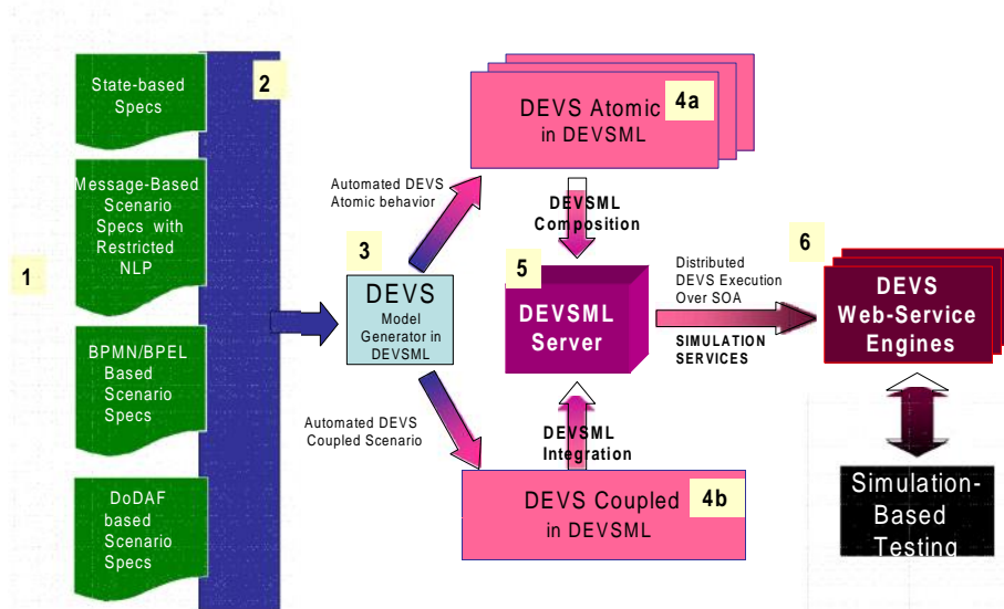
Figure 4: Net-centric collaboration and execution using DEVSML and DEVS/SOA
