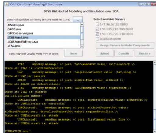
Figure 7: GUI snapshot of DEVS/SOA client hosting distributed simulation
