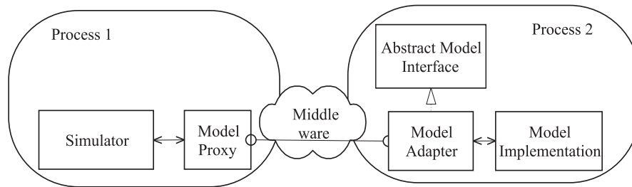
Figure 3. Adapting specific DEVS implementations to support the Abstract Model approach
