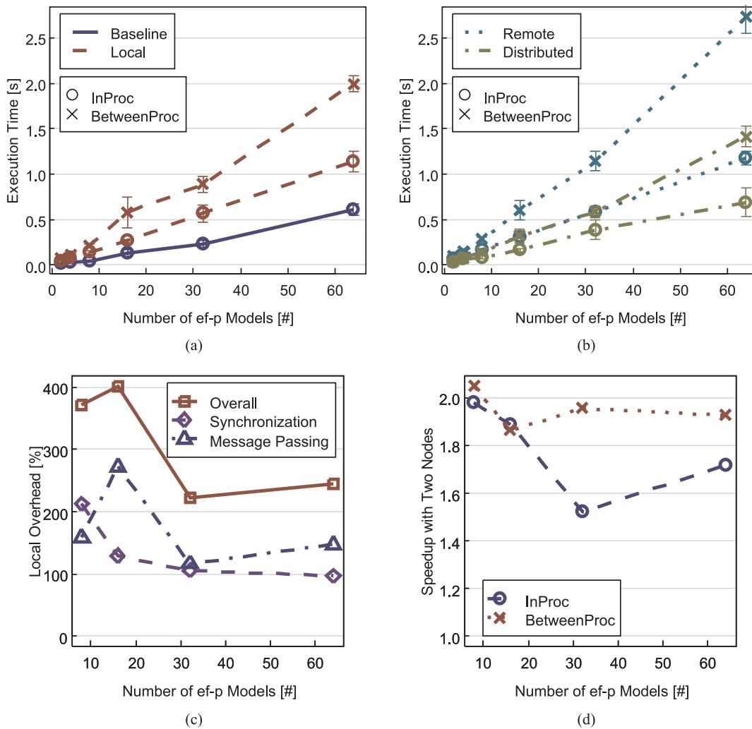
Figure 8. (a), (b) Execution times; (c) overheads; and (d) speedup of the performance experiments
