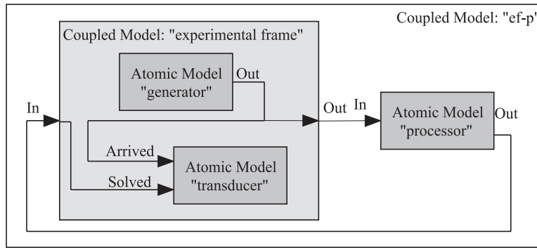
Figure 4. Experimental frame (ef)-processor (p) model
