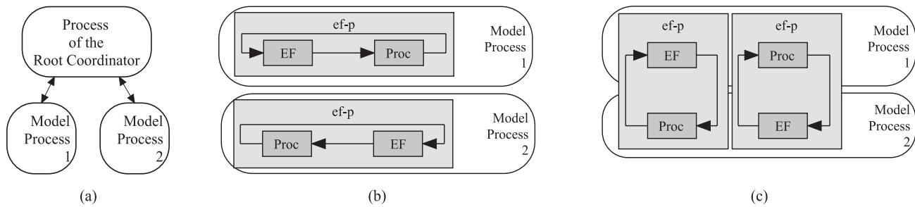
Figure 7. Allocation of model components to different operating system processes
