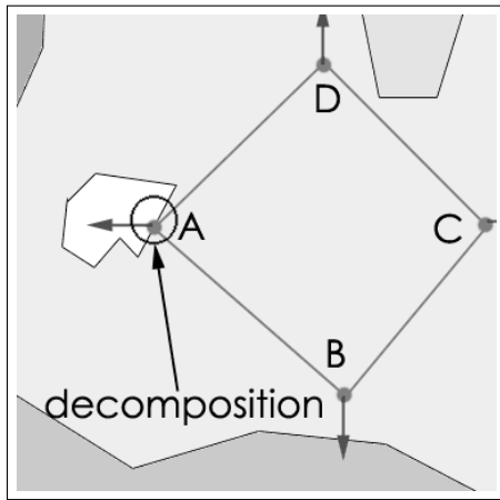
Figure 5: First collision.
