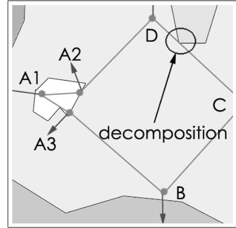
Figure 6: Second collision.
