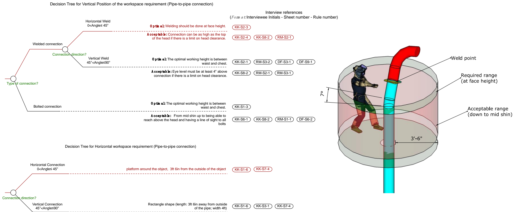
FIGURE 8: Decision tree for a pipe-to-pipe connection.
