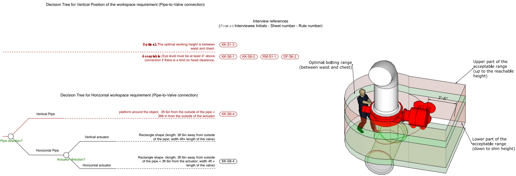
FIGURE 9: Decision tree for a valve-to-pipe connection
