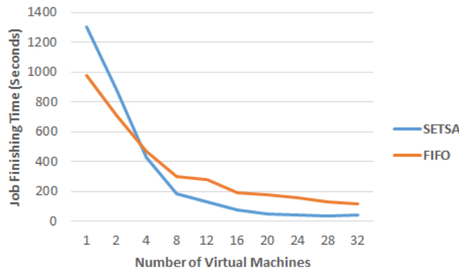
Figure 4. Performance of ASETS compared with FIFO scheduling in Amazon public cloud.
