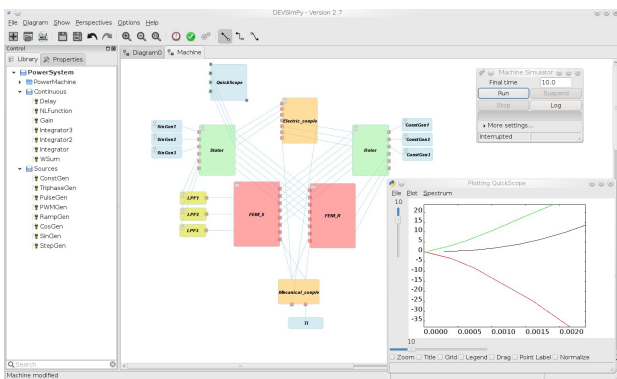
Figure 3. DEVSImPy general interface
