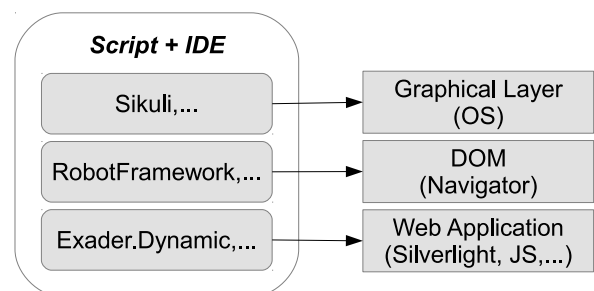
Figure 1. The three kinds of tools for web application testing
