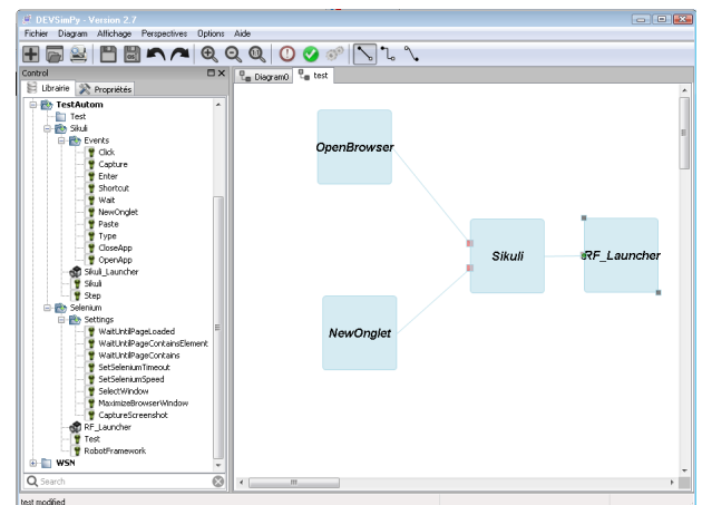
Figure 4. The TestAutom library with an example of use in DEVSImPy
