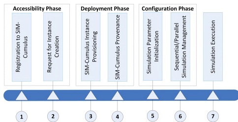
FIGURE 5. SIM-Cumulus workflow.
