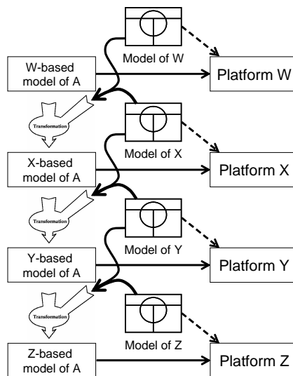
Fig. 12. Parameterization by Input & Output Platform Models
