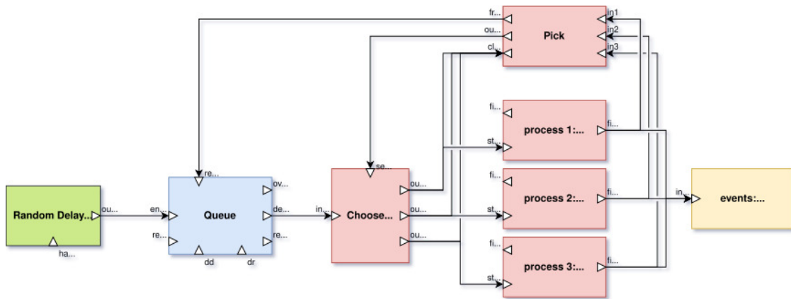
Figure 18: Example model using PythonPDEVS Building Block Library components
