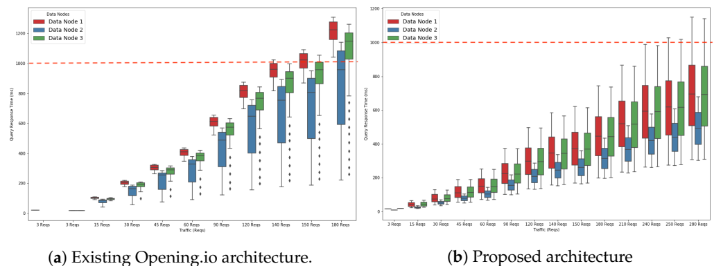
Figure 6. Comparison of query response time achieved with different query traffic volumes. The red dotted line represents the threshold (barrier) of 1 s, beyond which queries affect the response time of those received in the following second.
