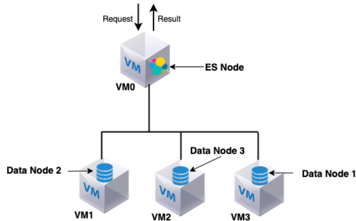
Figure 5. High level overview of the proposed revised Opening.io architecture.
