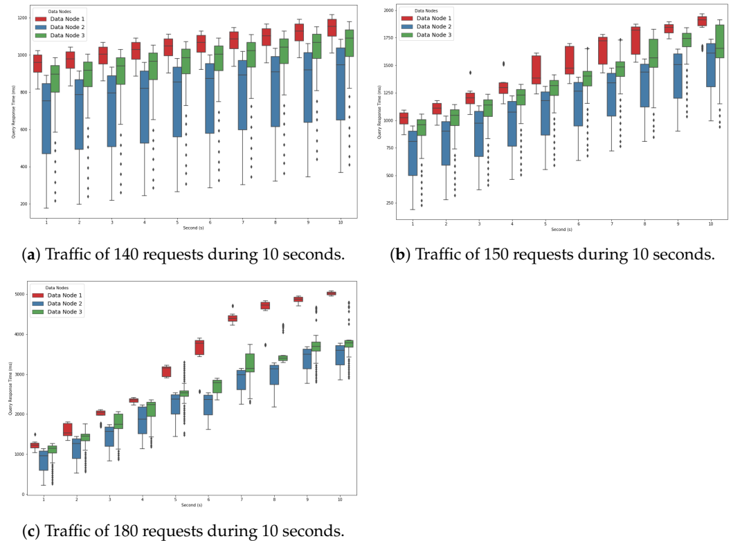
Figure 4. Query response time achieved for a traffic of (a) 140, (b) 150 and (c) 180 requests during 10 s.
