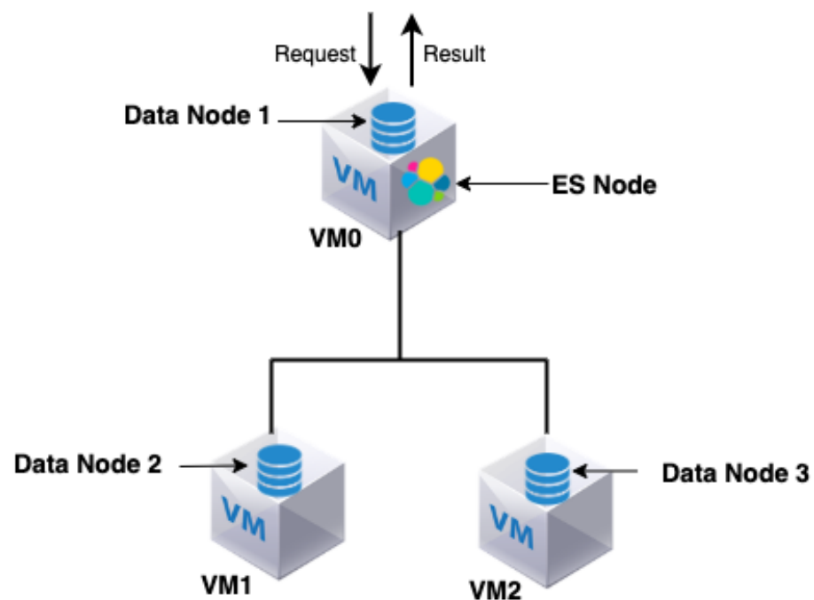
Figure 1. A high-level overview of the Opening.io architecture. VM: virtual machine; ES: Elasticsearch.
