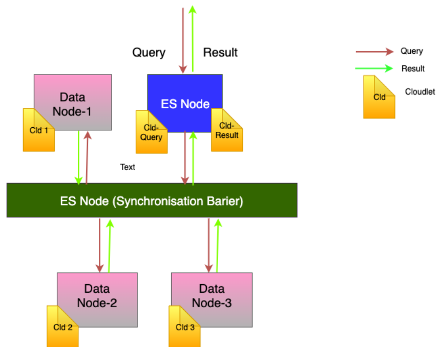
Figure 2. Modelling the application and workload propagation of Opening.io using the RECAP Discrete Event Simulator (DES).
