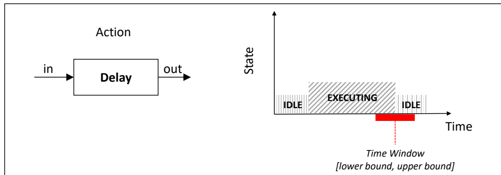
Figure 4: Modeling action-level as in activity-based modeling approach to enforce real-time constraints.
