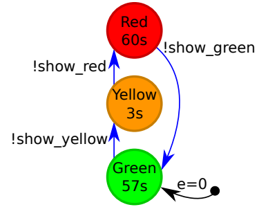
Figure 4: Model generating trace in Figure 3.
