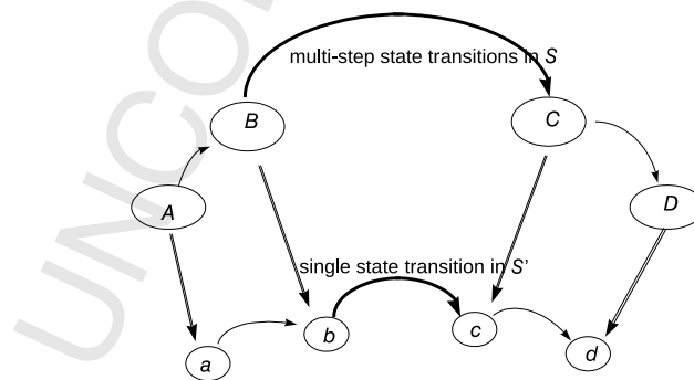
FIGURE 1.16 Homomorphism Concept. This figure illustrates the preservation of state transitions that a homomorphism requires.
