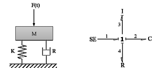
Figure 10: Mechanical Circuit and Bond-Graph
