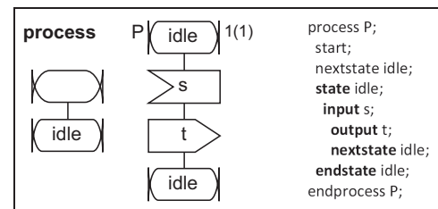
Figure 3. A non-graphical Specification and Description Language representation. In this example, the initial STATE is IDLE.
