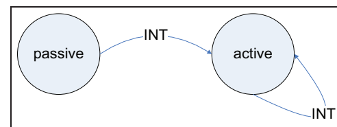
Figure 7. States diagram for the period Discrete Event System Specification model.
