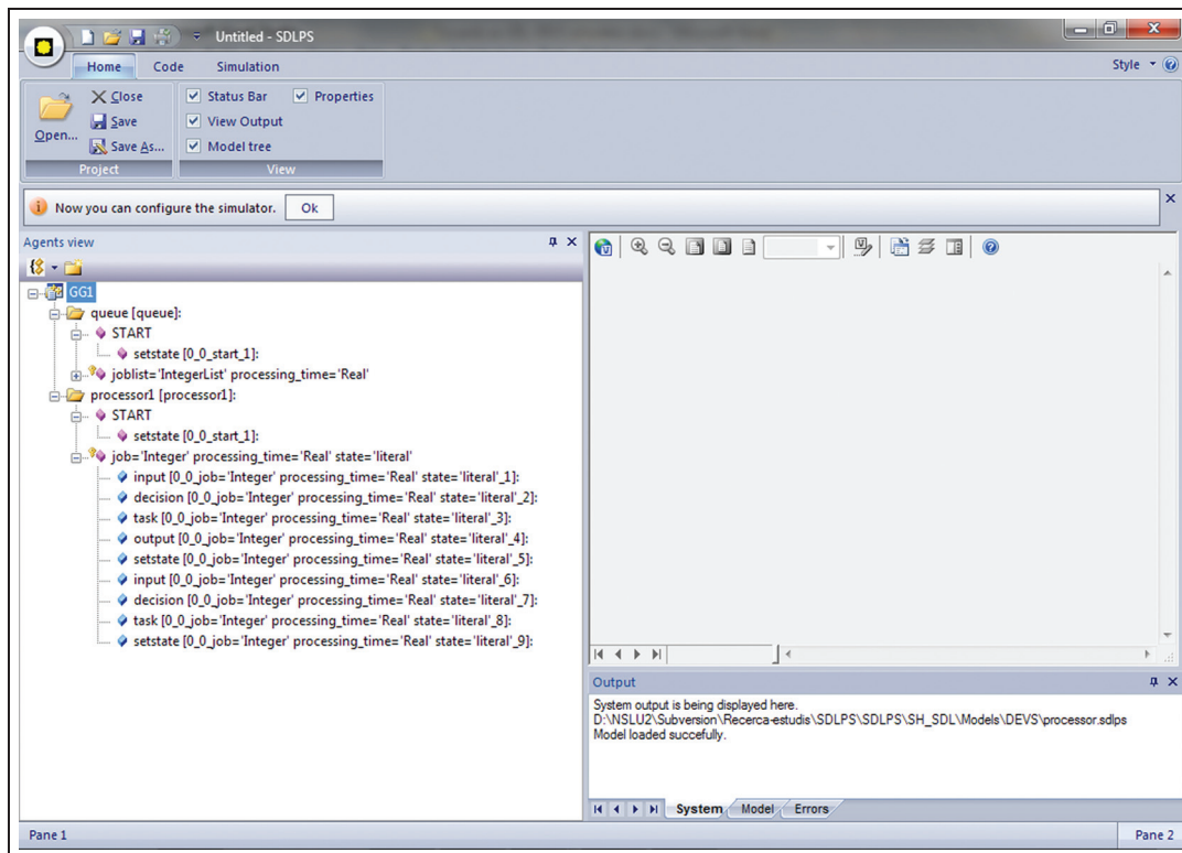
Figure 14. Specification and Description Language Parallel Simulator environment with the Discrete Event System Specification model loaded. The tree that contains all of the elements that define the model is on the left-hand side.
