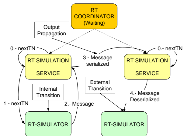
Figure 8: Real-time Communication among Services
