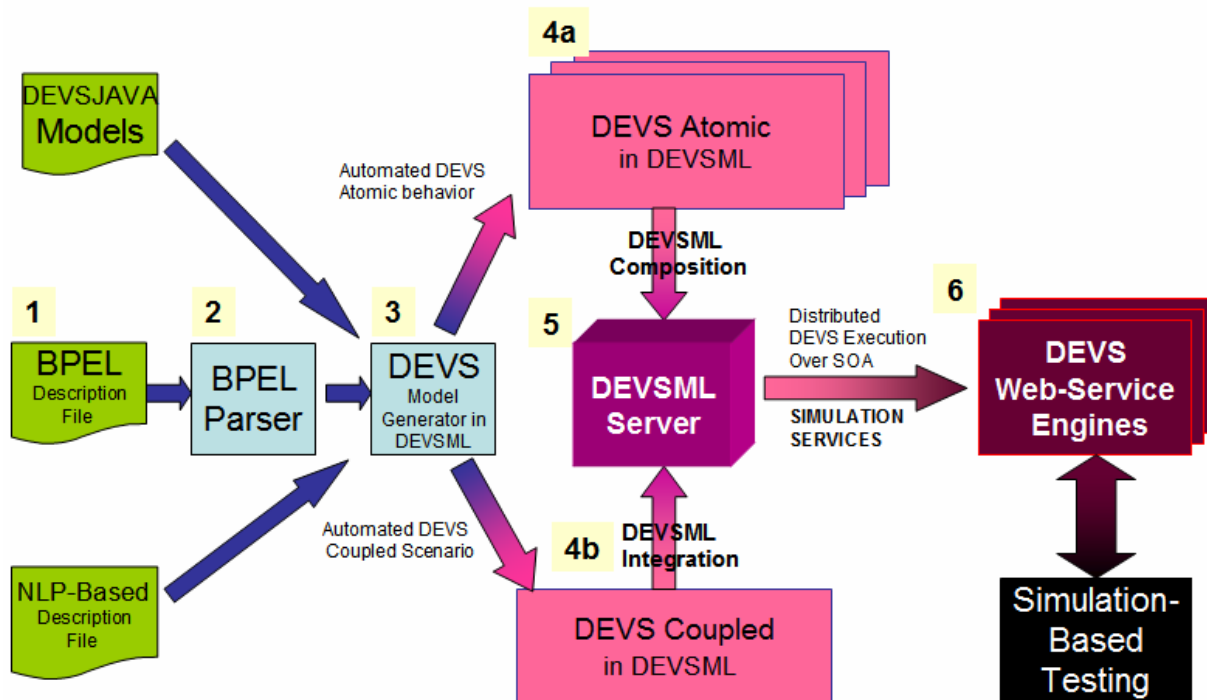
Figure 2: DEVSML and SOADEVs integrated
