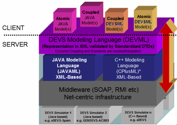
Figure 1: DEVMSML implementation over SOADEVs.
