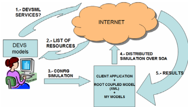
Figure 4: Execution of DEVS SOA-Based M&S
