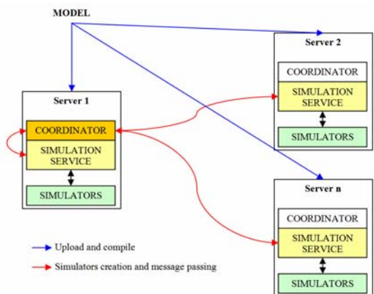
Figure 3: DEVMS/SOA distributed architecture
