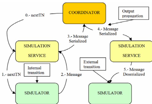
Figure 7: Centralized communication among services
