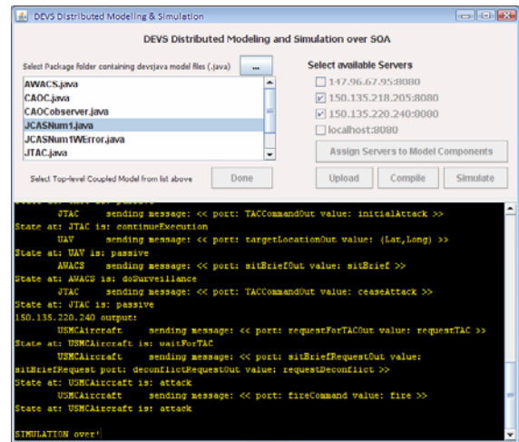
Figure 9: GUI snapshot of SOADEVs client hosting distributed simulation
