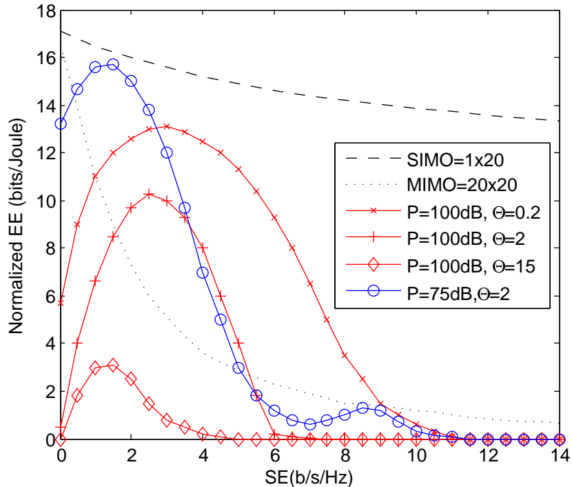
Fig. 5: Trade-off between EE and SE in cooperative virtual antenna array at the femtocell stage ( N_b = 2/Km , N_u = 30/Km , N_v = 300/Km ).
