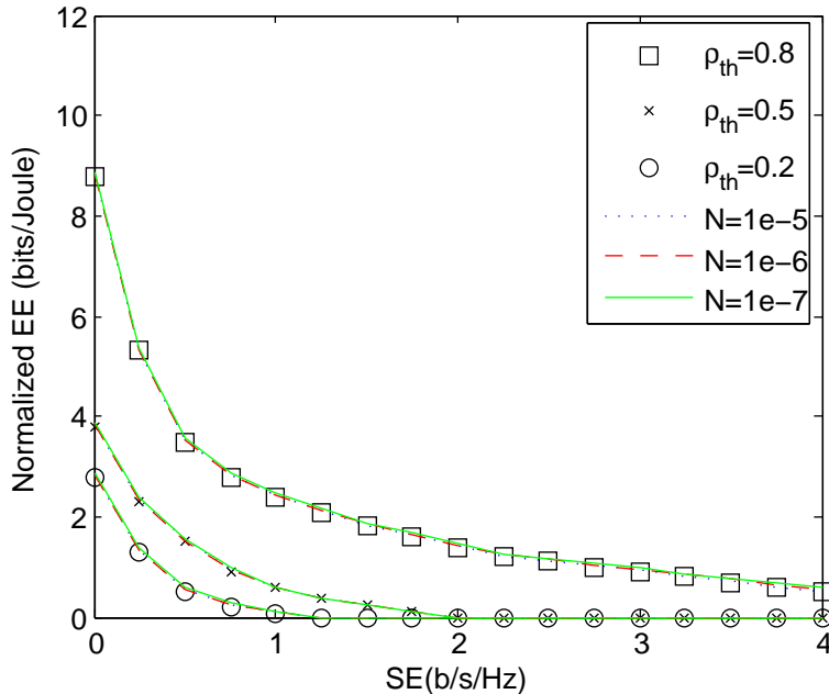
Fig. 4: The trade-off between EE and SE in CR femtocells at the network stage.
