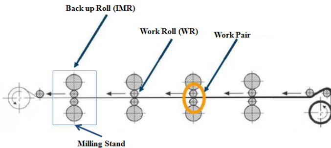
Figure 12. Roll Milling System [87]
