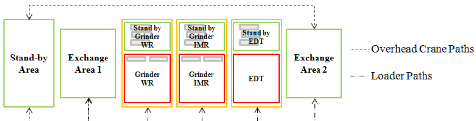
Figure 11. The Roll Shop System representation
