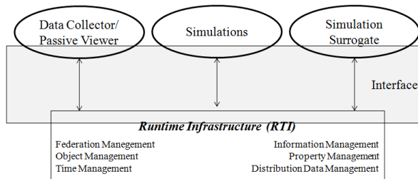
Figure 1. HLA Reference Architecture
