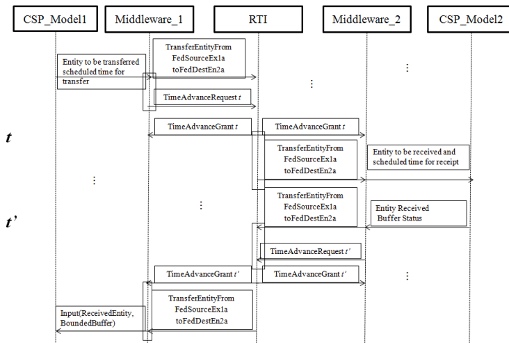
Figure 9. Communication Protocol
