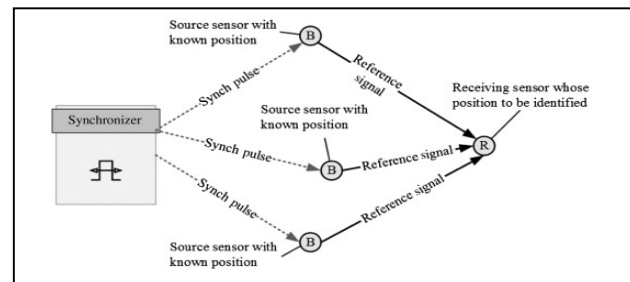
Fig.2. Time difference of arrival scheme.
