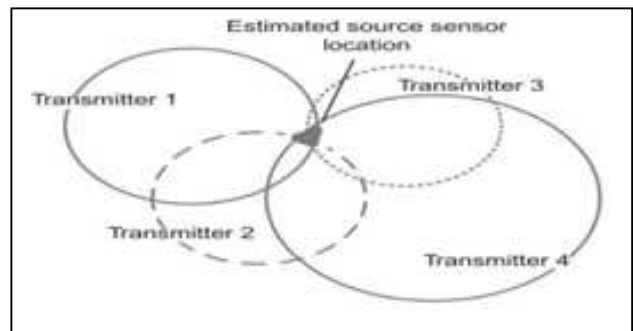
Fig. 1. TOA positioning system using multilateration
