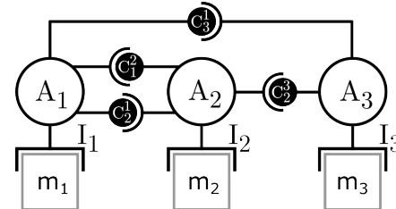
Figure 4. A multi-model described with AA4MM.
