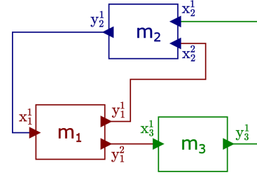
Figure 1. A multi-model composed of three models m_1 , m_2 and m_3 as a DEVS coupled model (here described with a simplified flattened version of DEVS).
