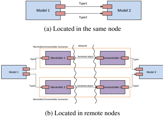
Figure 1: Marshaller/Unmarshaller Connectors
