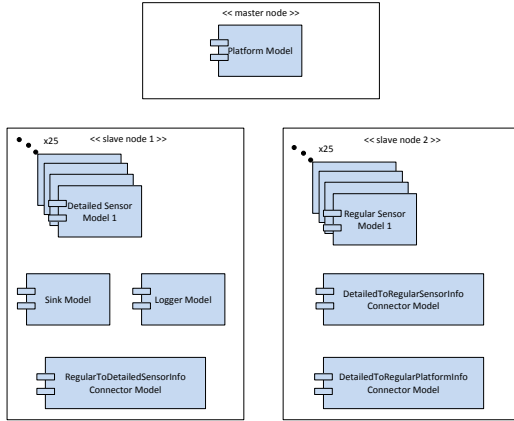
Figure 7: Partition Plan Overview of Case Study Scenario
