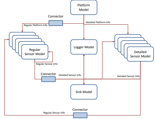
Figure 6: Models in the Case Study Scenario
