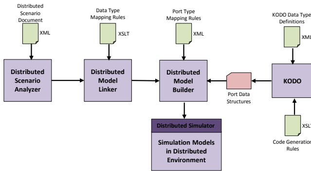
Figure 4: Distributed SiMA Simulation Construction Pipeline
