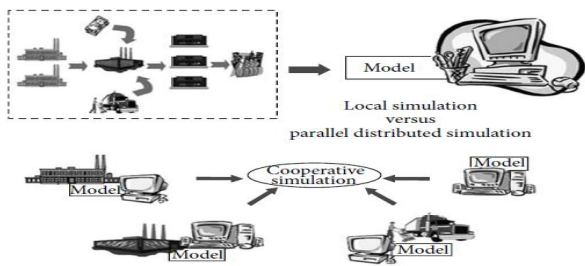
Figure 2: The two paradigms for SCM simulation.
