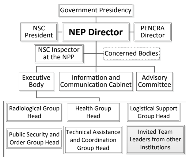
Figure 1. NEP structure
