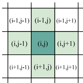
(a) von Neumann neighborhood (r = 1).
