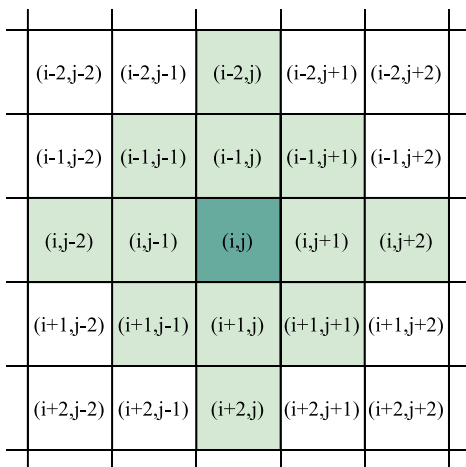
(c) von Neumann neighborhood (r = 2).
