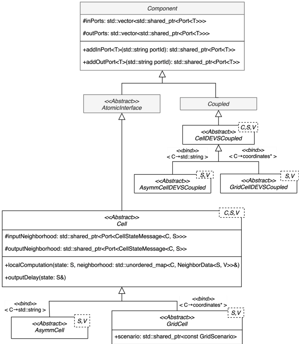
Fig. 9. Simplified UML class diagram of the Cadmium Cell-DEVS library.
