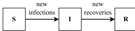
Fig. 1. Schematic of the SIR compartmental model.
