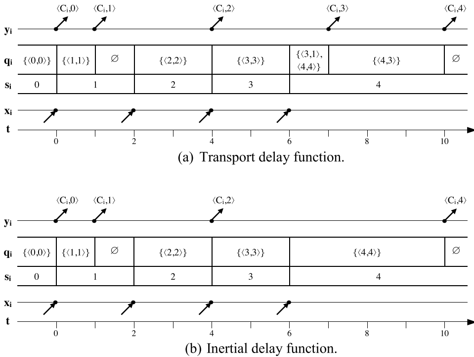
Fig. 6. Comparison of transport and inertial delay functions.
