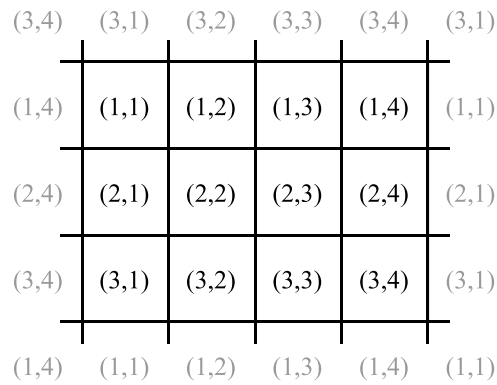
Fig. 2. Example of classic cellular model.
