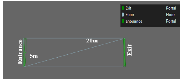
Fig. 3 - Scenario design.
