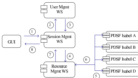
Figure 5. Steps to Launch an Isabel Session
