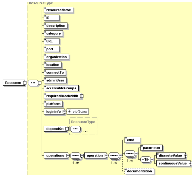
Figure 2. Resource Schema
