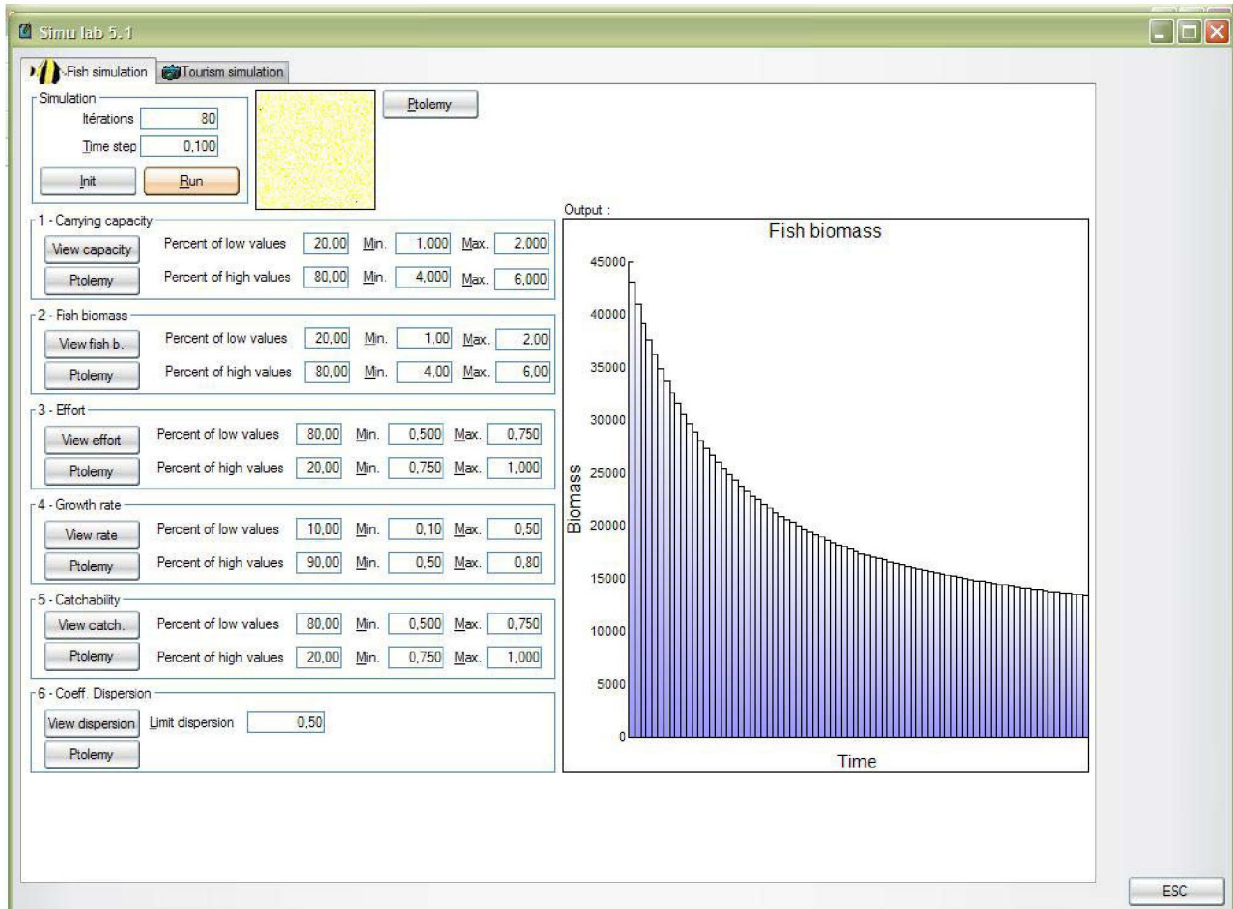
Fig. 4. Interface snapshot
