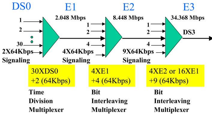
Figure 2.6 European hierarchy.
