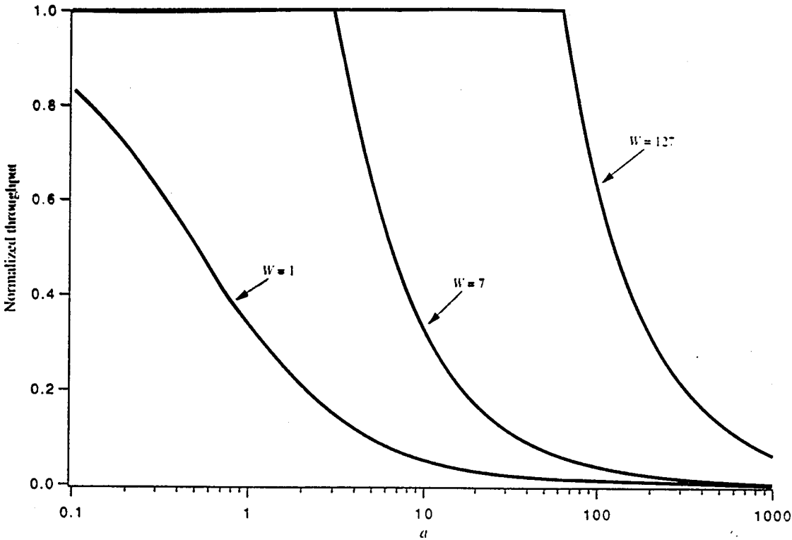
Figure 9.11 Sliding-window throughput as a function of a .
