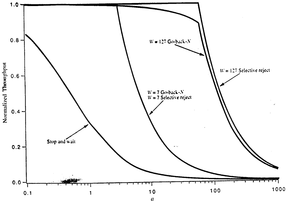
Figure 9.12 ARQ throughput as a function of \alpha ( P = 10^{-3} ).
