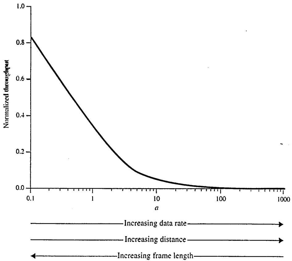
Figure 9.9 Performance of stop-and-wait protocol ( P = 10^{-3} ).
