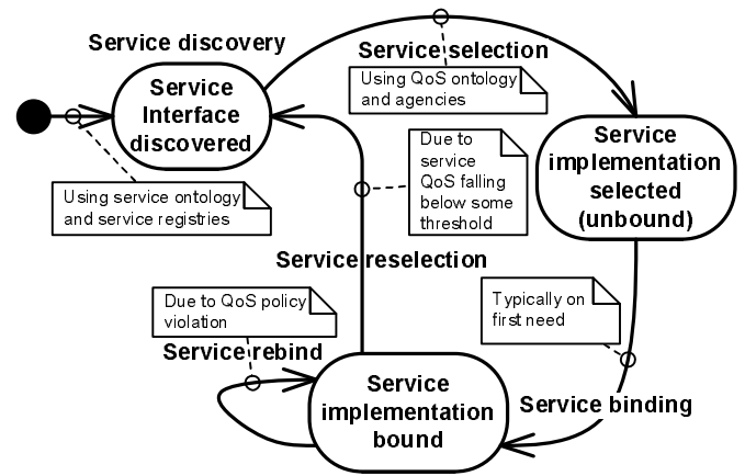
Figure 1: Service instance usage life-cycle.
