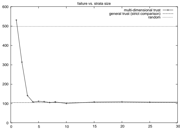
Figure 1: Failure rate for MDT versus strata.
