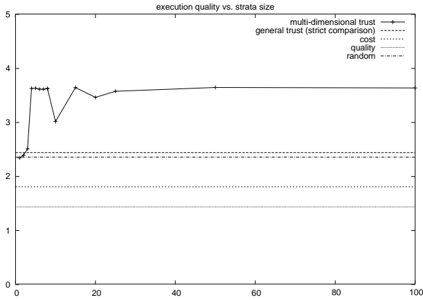
Figure 3: Execution quality for MDT versus strata.
