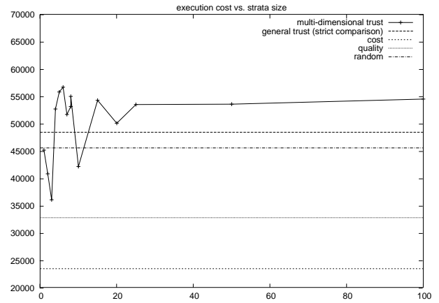
Figure 2: Execution cost for MDT versus strata.
