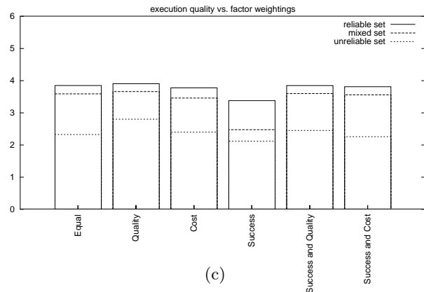
Figure 4: Failure rate (a), execution cost (b) and execution quality (c) for selected factor weightings in reliable, mixed, and unreliable contexts.
