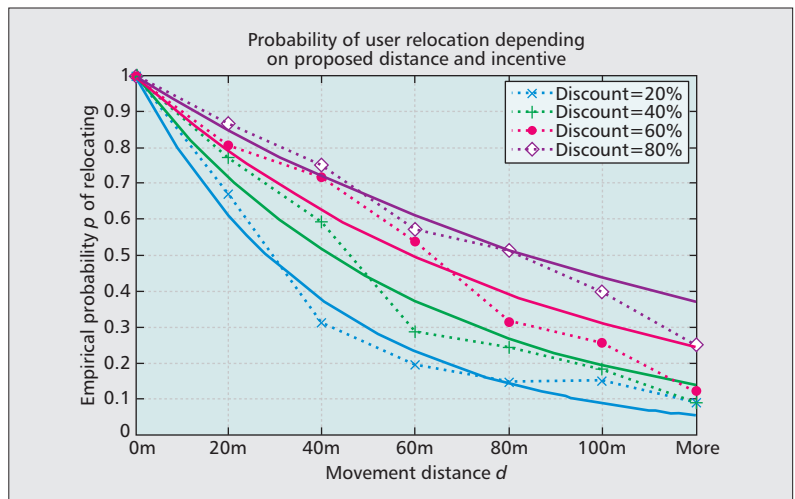
Figure 5. This figure shows the reaction ( p_S ) to relocation suggestions (proposed distance d ) with different discount incentives for data traffic [8]. The solid lines are exponential fits. Moving within a small distance is easily accepted. Moving more requires an incentive or a good reason.
